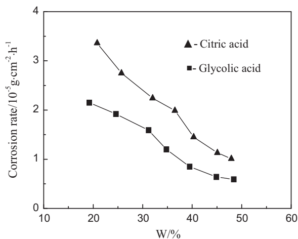
Fig. 9. Relationship between the W-content and the corrosion rate of the Ni–W coatings in 10% H 2 SO 4 solution.
