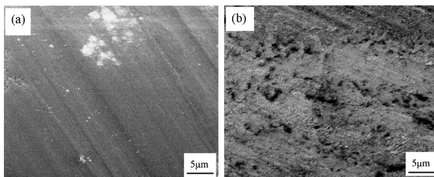
Fig. 7. The worn morphologies of Ni–W coatings.
