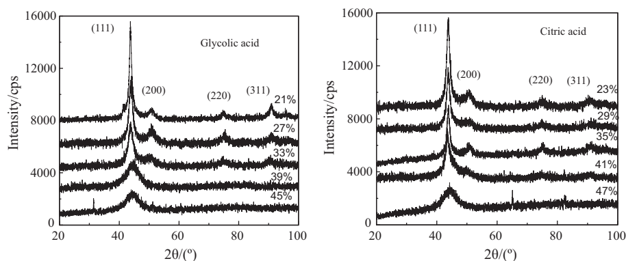
Fig. 3. XRD spectra patterns of Ni-W coatings with different W-contents.
