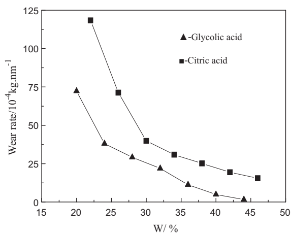
Fig. 5. Relationship between the W-content in the coatings and the wear rate of the coatings.
