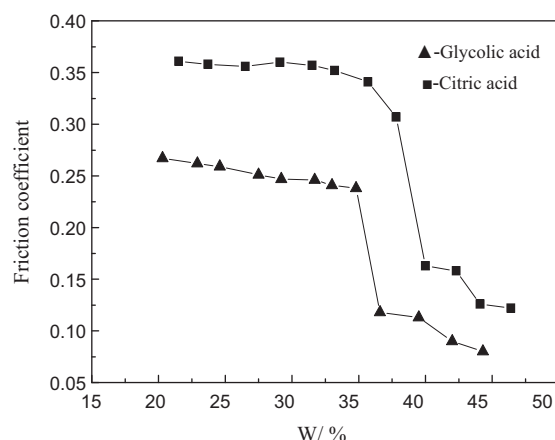
Fig. 6. Relationship between the W-content in the coatings and the friction coefficient of the coatings.
