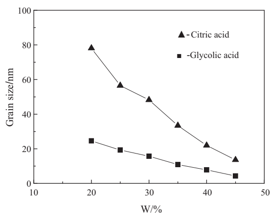
Fig. 4. The grain size of matrix Ni in the coatings.
