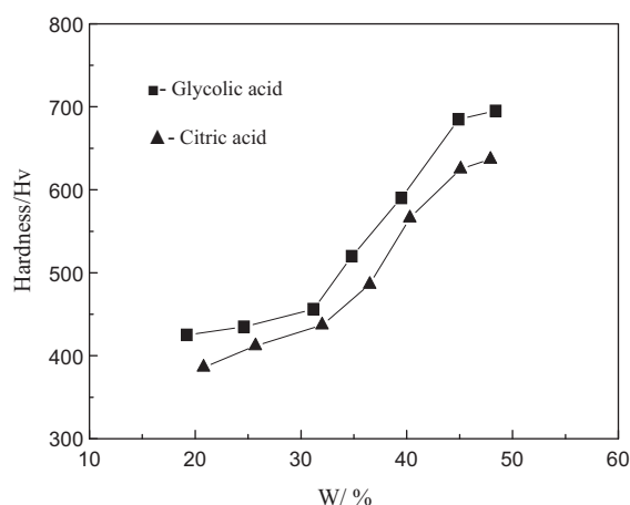
Fig. 8. Relationship between the W-content in the coatings and the hardness of the coatings.
